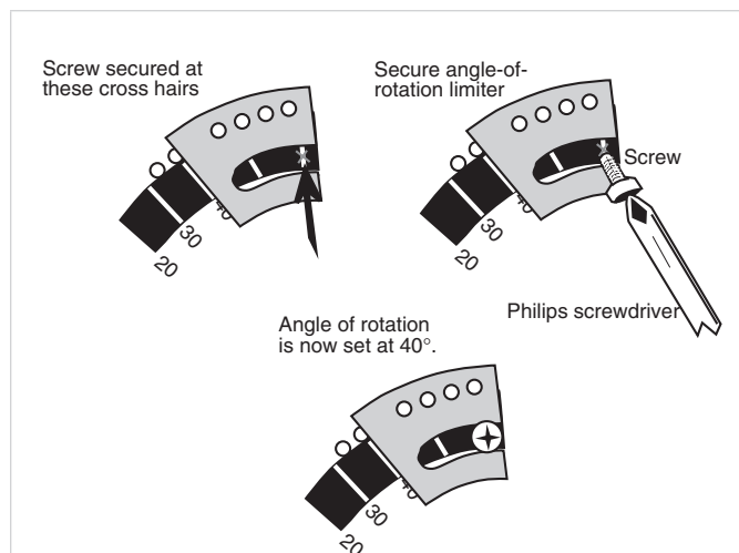
FIGURE C – ZDB-AF2 US, Securing the Angle of Rotation Limiter
