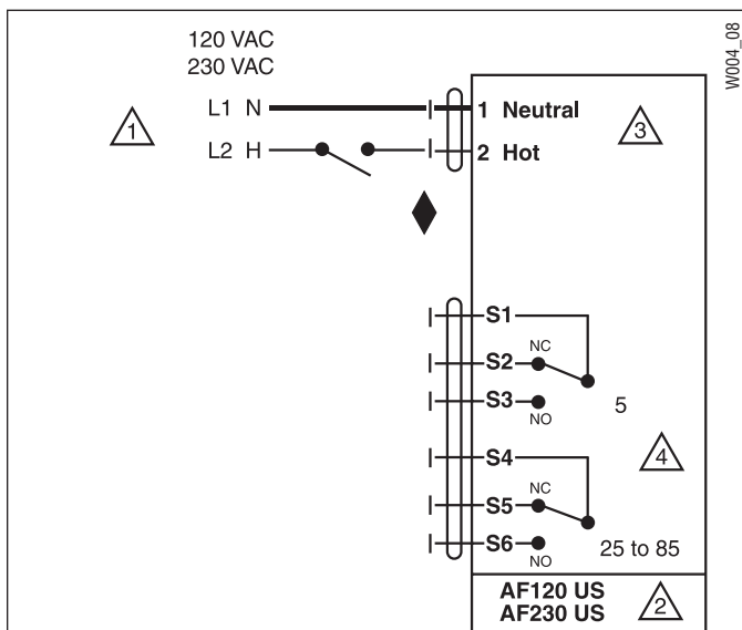
On/Off wiring for AF120-S US and AF230-S US
