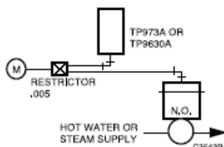
TP973 Typical Piping (One-pipe)
