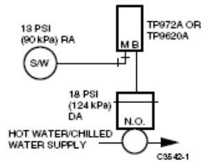
TP972 Typical Piping
