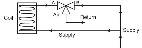
3-way Mixing Valve Piping Diagram
